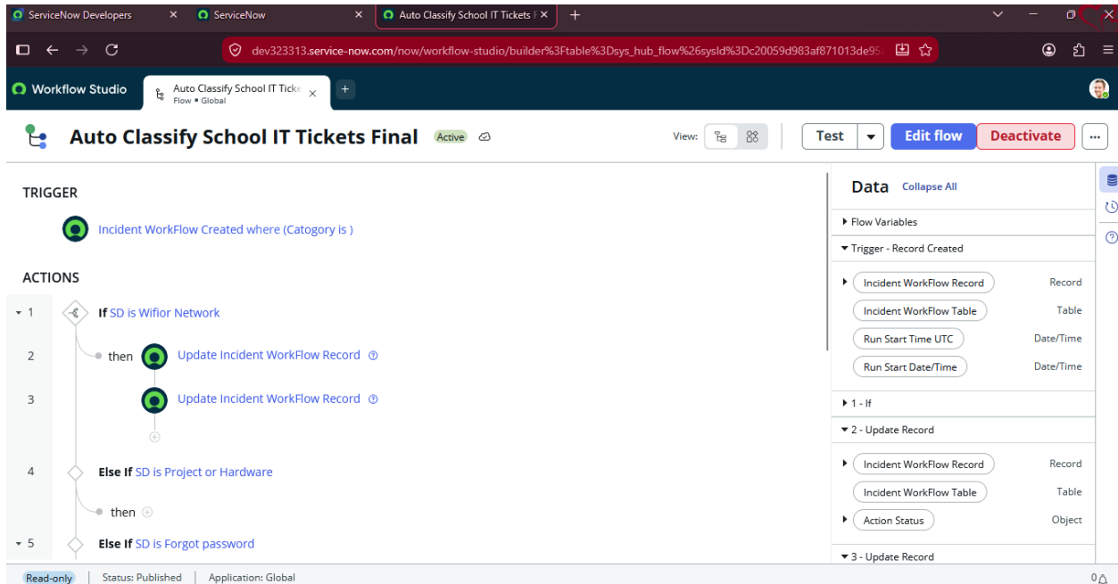
Figure 1. Flow Designer showing the active Auto Classify School IT Tickets workflow, record-created trigger and conditional actions.
